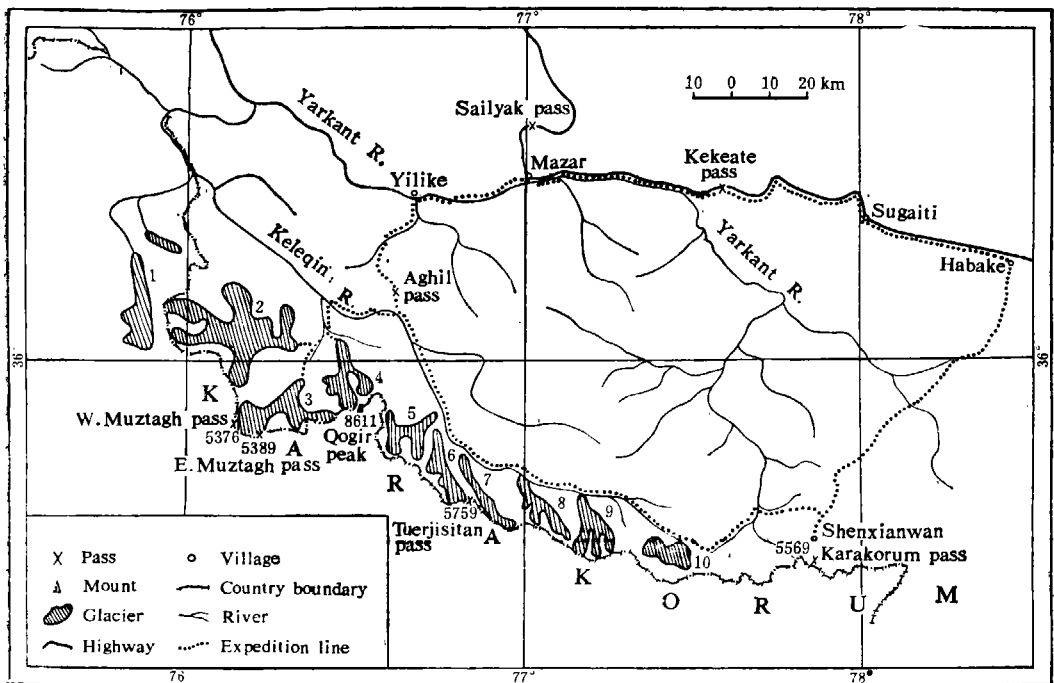
Fig. 1. The distribution of the big glaciers in the Keleqin River on the northern slope of the Karakorum Mountains.
