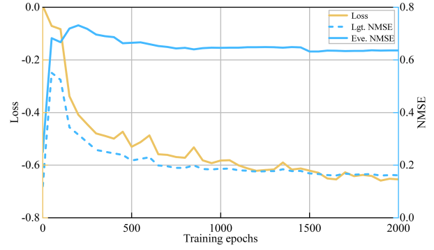
图4 (网络版彩图) 深度展开 GNN 的训练收敛。 Figure 4 (Color online) Convergence of unfolded GNN training.
