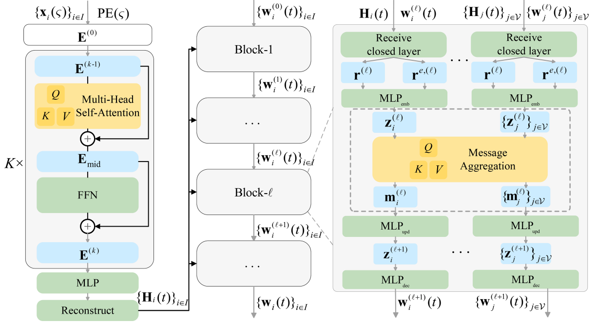
图 2 (网络版彩图) “预测 – 决策” 求解框架 (基于时序 Transformer 的预测与基于深度展开 GNN 的 AirComp 决策). Figure 2 (Color online) The “prediction-decision” framework (temporal Transformer for channel prediction and unfolled GNN for AirComp strategy).
