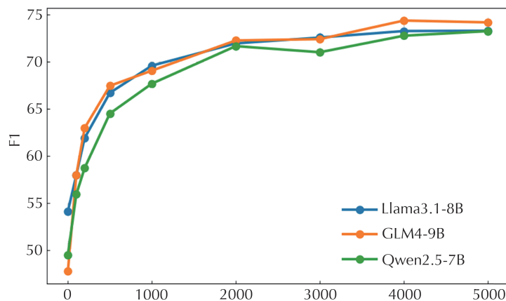
Figure 3. Performance comparison of different LLM backbones with varying training dataset sizes.
