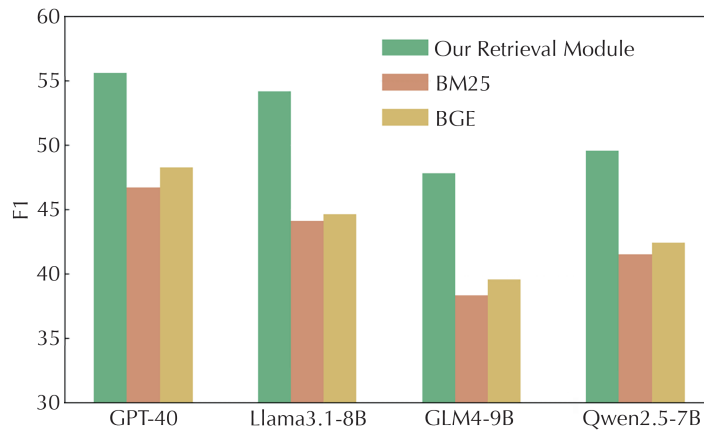
Figure 2. Performance comparison of different Retrieval Modules.
